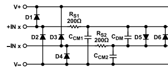
Figure 72. Input EMI Filter and Clamp Circuit
