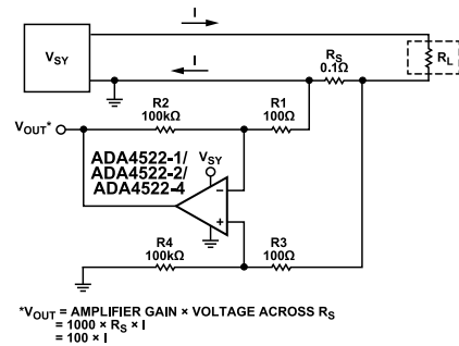
Figure 84. Low-Side Current Sensing Circuit
