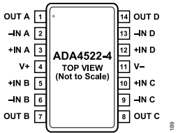
Figure 5. ADA4522-4 Pin Configuration
