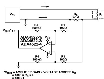
Figure 84. Low-Side Current Sensing Circuit
