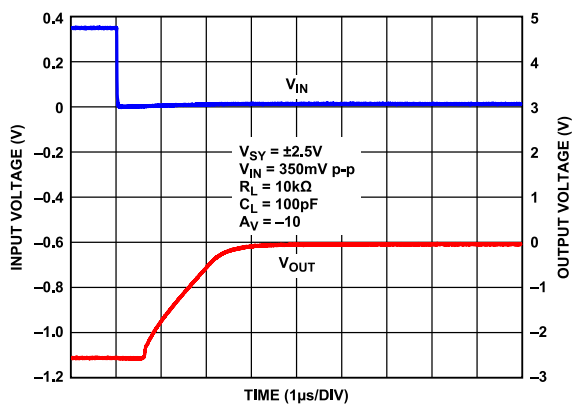
Figure 57. Negative Overload Recovery, V_{SY} = \pm 2.5V
