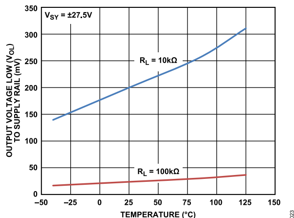
Figure 29. Output Voltage Low ( V_{OL} ) to Supply Rail vs. Temperature, V_{SY} = \pm 27.5\text{ V}
