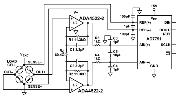
Figure 83. Precision Weigh Scale Measurement System
