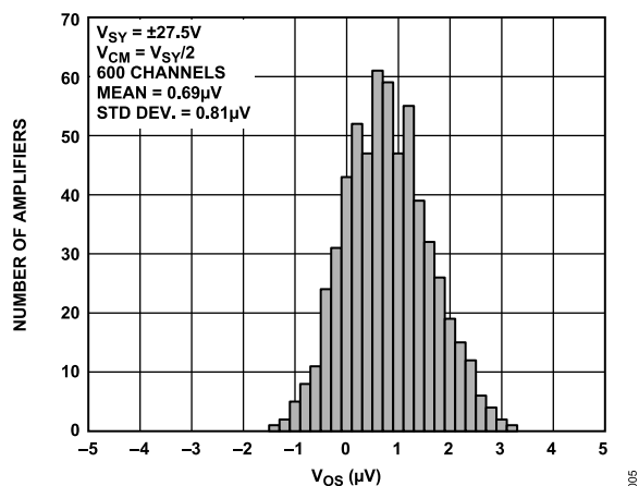
Figure 8. Input Offset Voltage Distribution, V_{SY} = \pm 27.5\text{ V}
