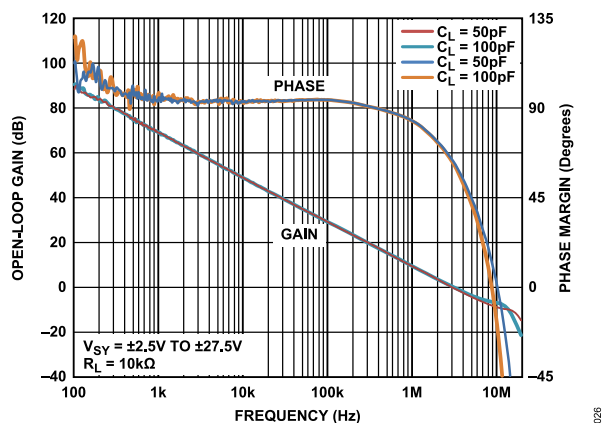
Figure 32. Open-Loop Gain and Phase Margin vs. Frequency
