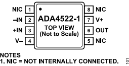
Figure 3. ADA4522-1 Pin Configuration
