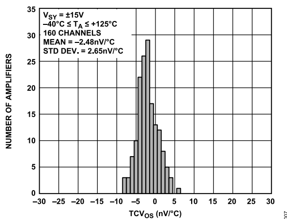
Figure 10. Input Offset Voltage Drift Distribution, V_{SY} = \pm 15\text{ V}
