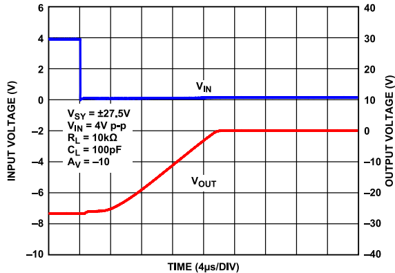
Figure 59. Negative Overload Recovery, V_{SY} = \pm 27.5V
