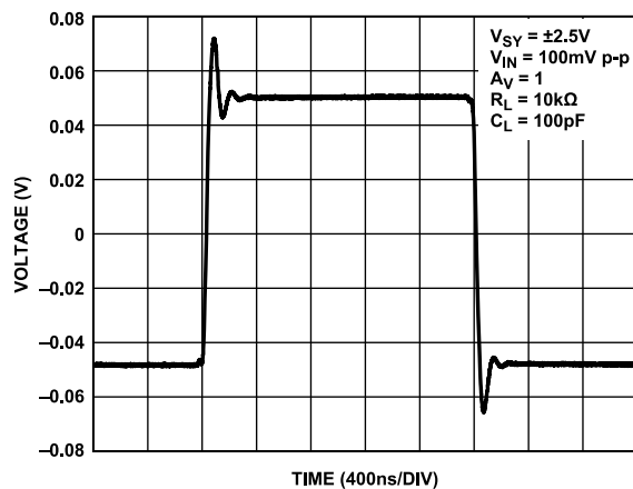
Figure 39. Small Signal Transient Response, V_{SY} = \pm 2.5V
