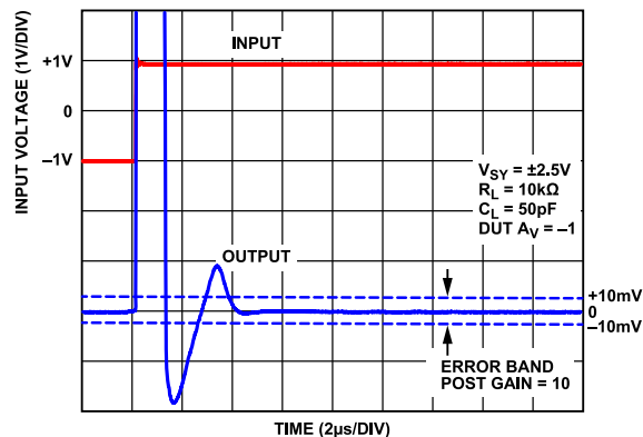
Figure 69. Positive Settling Time to 0.1%, V_{SY} = \pm 2.5V
