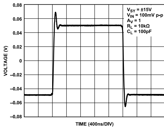
Figure 40. Small Signal Transient Response, V_{SY} = \pm 15V
