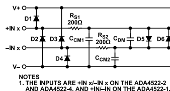
Figure 72. Input EMI Filter and Clamp Circuit
