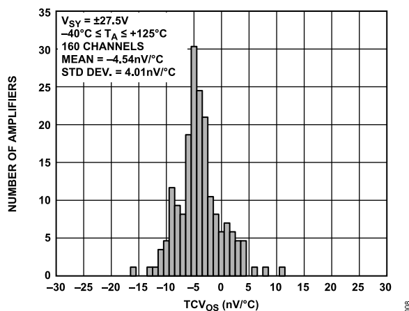
Figure 11. Input Offset Voltage Drift Distribution, V_{SY} = \pm 27.5\text{ V}
