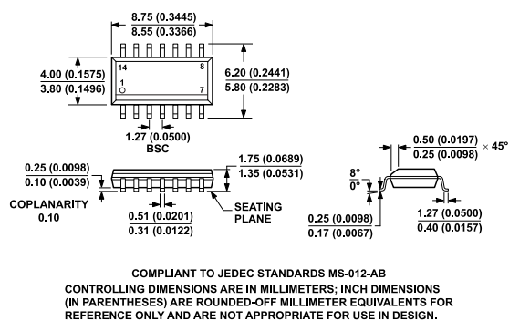
Figure 92. 14-Lead Small Outline Package [SOIC_N] Narrow Body (R-14) Dimensions shown in millimeters and (inches)
