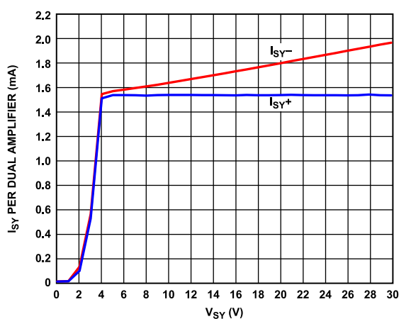
Figure 88. Supply Current ( I_{SY} ) per Dual Amplifier vs. Supply Voltage ( V_{SY} ) (ADA4522-1/ADA4522-2/ADA4522-4 as a Comparator)
