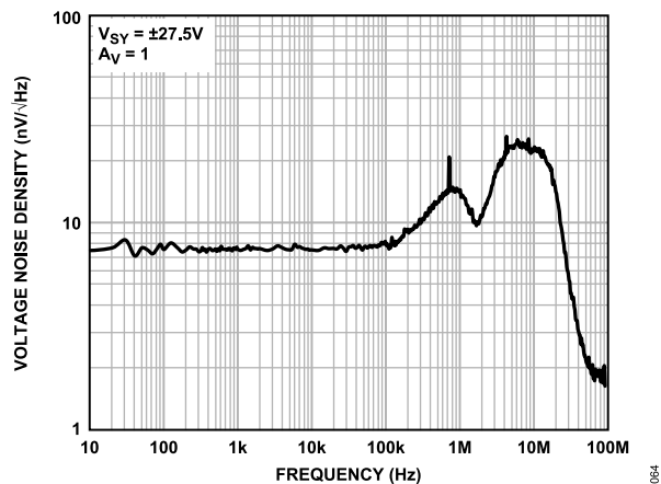
Figure 62. Voltage Noise Density vs. Frequency, V_{SY} = \pm 27.5\text{ V}
