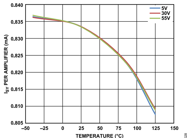
Figure 34. Supply Current ( I_{SY} ) per Amplifier vs. Temperature
