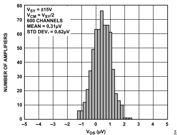
Figure 7. Input Offset Voltage Distribution, V_{SY} = \pm 15\text{ V}
