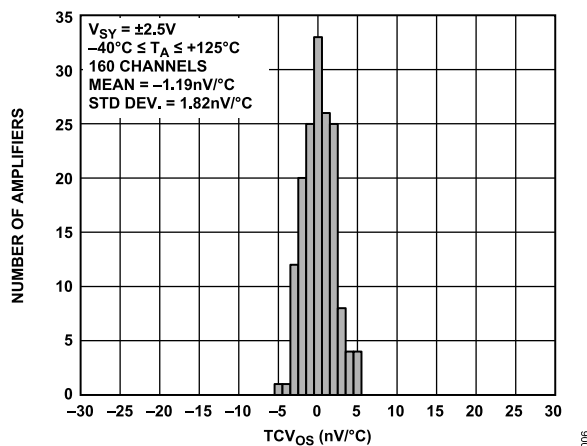
Figure 9. Input Offset Voltage Drift Distribution, V_{SY} = \pm 2.5\text{ V}
