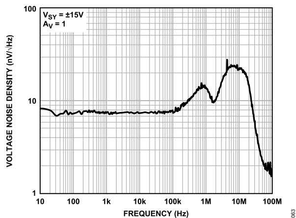
Figure 61. Voltage Noise Density vs. Frequency, V_{SY} = \pm 15\text{ V}
