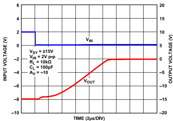
Figure 58. Negative Overload Recovery, V_{SY} = \pm 15V
