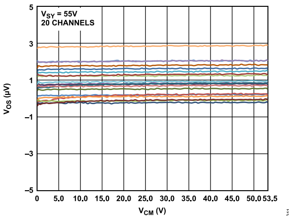
Figure 14. Input Offset Voltage ( V_{OS} ) vs. Common-Mode Voltage ( V_{CM} ), V_{SY} = 55V
