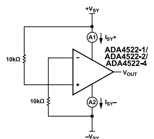
Figure 87. Comparator Configuration B
