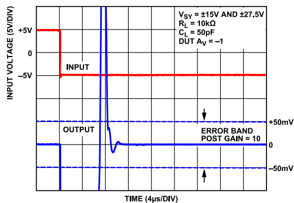
Figure 70. Positive Settling Time to 0.1%, V_{SY} = \pm 15V and \pm 27.5V
