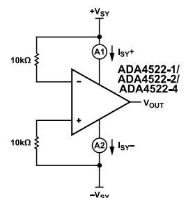
Figure 86. Comparator Configuration A
