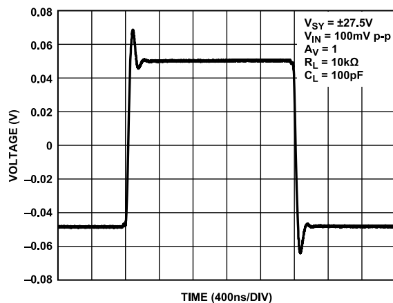
Figure 41. Small Signal Transient Response, V_{SY} = \pm 27.5V
