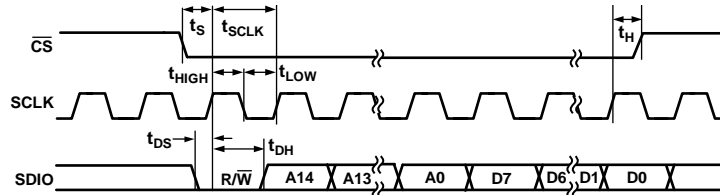
Figure 3. SPI Write Operation Timing
