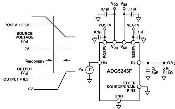
Figure 41. Overvoltage Recovery Time, t_{RECOVERY}
