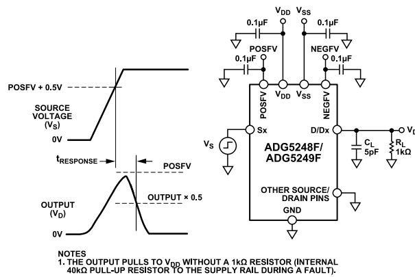
Figure 43. Overvoltage Response Time, t_{RESPONSE}
