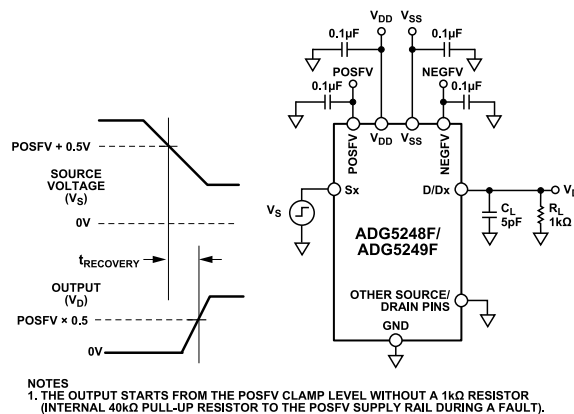
Figure 44. Overvoltage Recovery Time, t_{RECOVERY}
