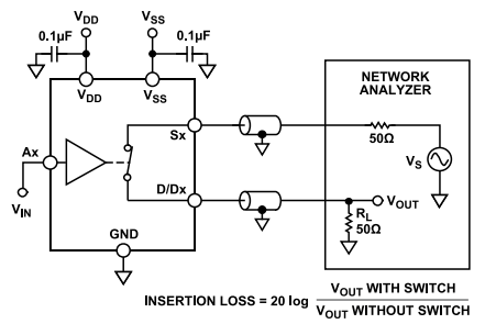
Figure 42. Bandwidth
