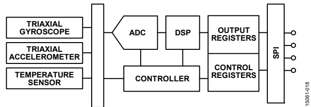
Figure 26. Basic Operation
