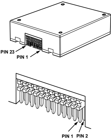
Figure 8. Axial Orientation (Top Side Facing Up)
