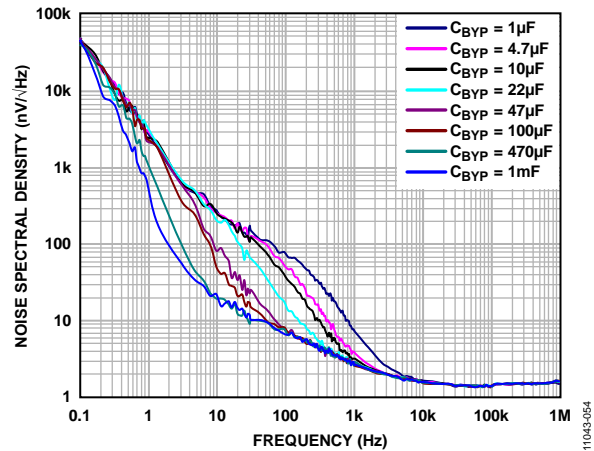
Figure 54. Noise Spectral Density vs. Frequency, C_{BYP} = 1\ \mu\text{F} to 1 mF
