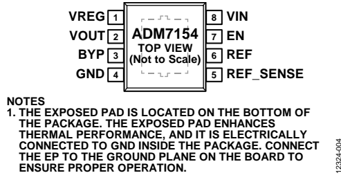
Figure 4. 8-Lead SOIC Pin Configuration
