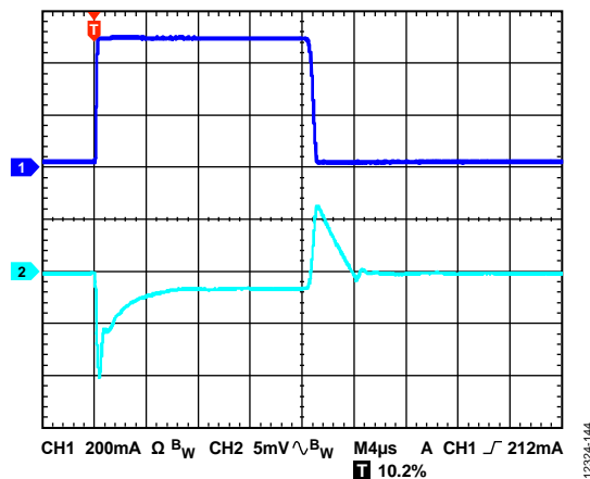
Figure 44. Output Transient Response, V_{\text{OUT}} = 3.3\text{ V} , C_{\text{OUT}} = 10\ \mu\text{F} , CH1 = Load Current, CH2 = V_{\text{OUT}}
