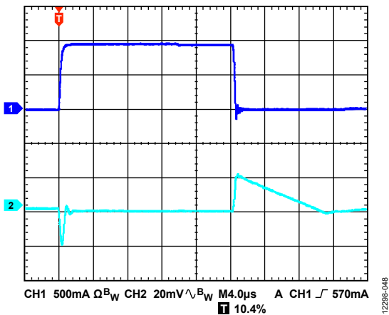
Figure 48. Load Transient Response, I_{LOAD} = 10 \text{ mA} to 1 \text{ A} , V_{OUT} = 5 V , V_{IN} = 5.5 V , CH1 = I_{LOAD} , CH2 = V_{OUT}
