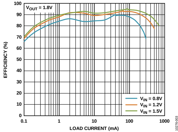
Figure 3. Auto Mode Efficiency vs. Load Current, V_{OUT} = 1.8\text{ V}
