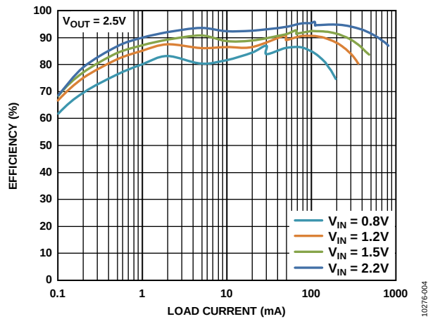
Figure 4. Auto Mode Efficiency vs. Load Current, V_{OUT} = 2.5\text{ V}
