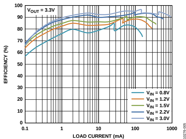
Figure 5. Auto Mode Efficiency vs. Load Current, V_{OUT} = 3.3\text{ V}
