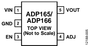
Figure 5. 5-Lead TSOT, Adjustable Output Pin Configuration
