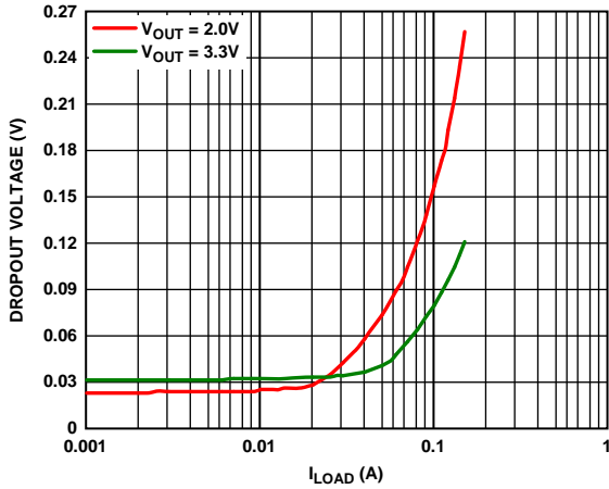
Figure 16. Dropout Voltage vs. Load Current ( I_{LOAD} )
