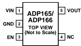
NOTES 1. NC = NO CONNECT. NOT CONNECTED INTERNALLY. 12188-004 Figure 4. 5-Lead TSOT, Fixed Output Pin Configuration
