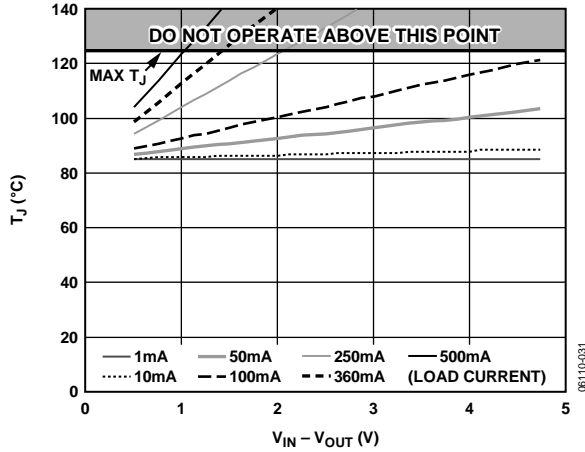
Figure 43. 300 mm 2 of PCB Copper, T A = 85°C
