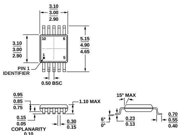
Figure 92. 10-Lead Mini Small Outline Package [MSOP] (BM-10)
