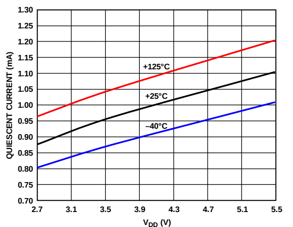
Figure 63. Quiescent Current vs. V_{DD} ( V_{IN} = 13 V)
