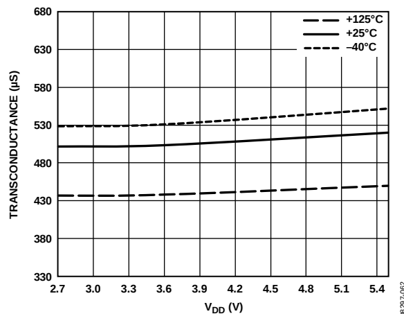
Figure 62. Transconductance ( G_M ) vs. V_{DD}
