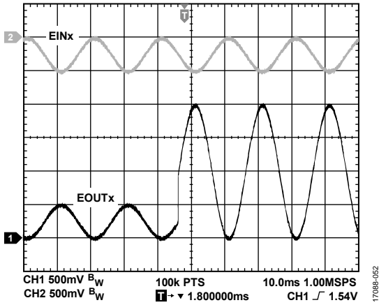
Figure 53. PGA Gain Switching from Gain = 1 to Gain = 4
