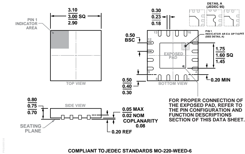
Figure 64. 16-Lead Lead Frame Chip Scale Package [LFCS] 3 mm × 3 mm Body and 0.75 mm Package Height (CP-16-22) Dimensions shown in millimeters
