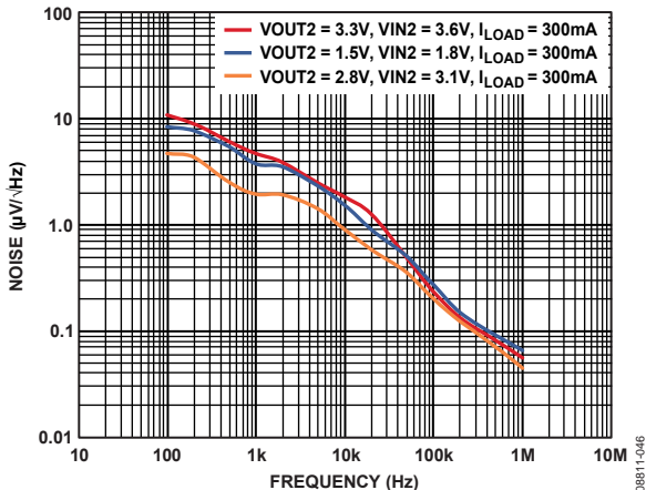
Figure 47. LDO1 Noise Spectrum Across Output Voltage, V_{IN} = V_{OUT} + 0.3 V
