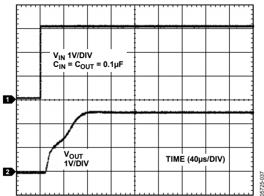
Figure 33. ADR121 Turn-On Response
