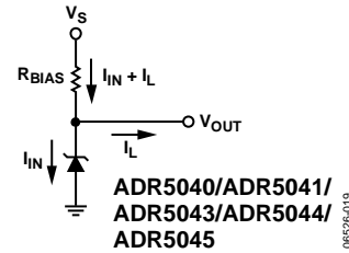
Figure 19. Shunt Reference
