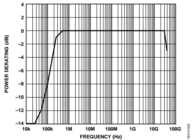
Figure 2. Power Derating for Through Path and Hot Switching vs. Frequency, T CASE = 85°C
