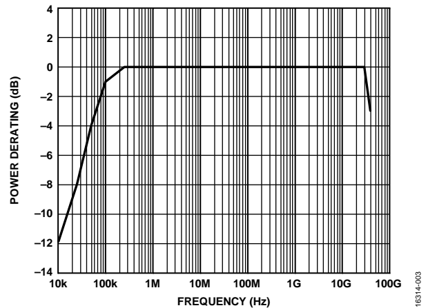
Figure 3. Power Derating for Terminated Path vs. Frequency, T CASE = 85°C
