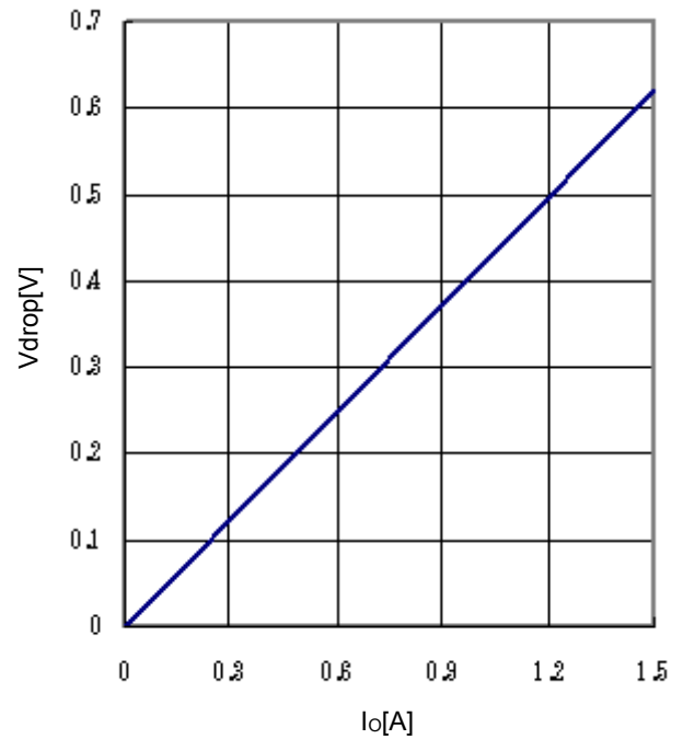
Fig.22 Minimum dropout Voltage 2 ( V_{cc}=4.5 V, T_a=25 °C)
