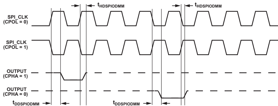
Figure 44. ODM Master
