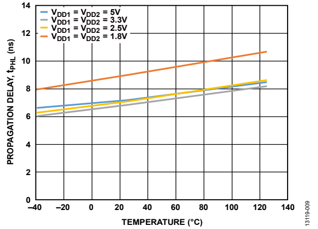
Figure 20. Propagation Delay, t_{PHL} vs. Temperature at Various Voltages
