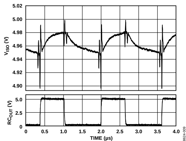
Figure 10. Typical Output Voltage Ripple at 90% Load, V_{ISO} = 5 V
