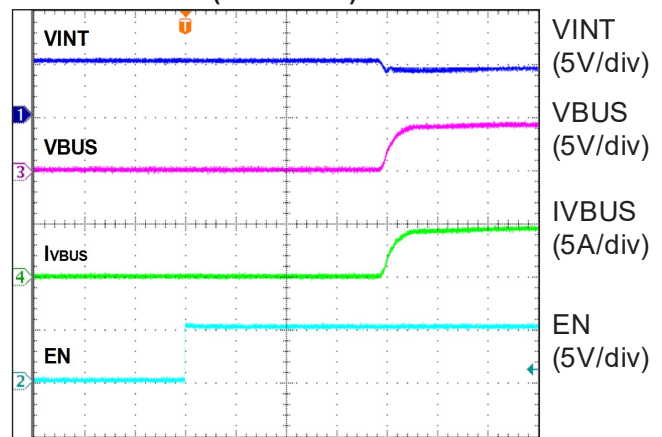
Turn-On by EN (VINT = 5V)
