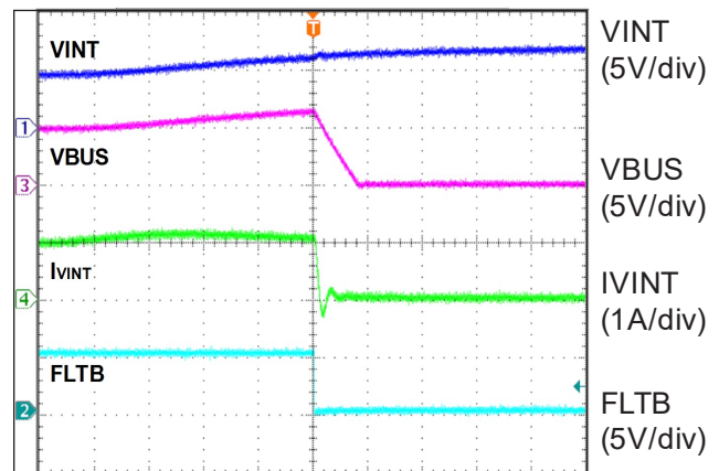
VINT OVP Operation with R_{OVP} = 301\text{k}\Omega
