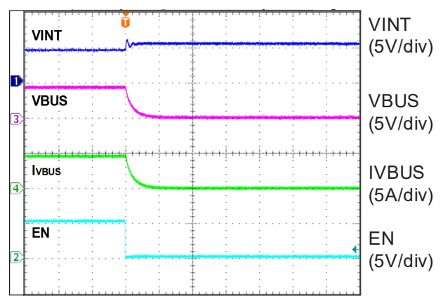
Turn-Off by EN (VINT = 5V)
