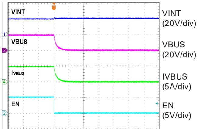
Turn-Off by EN (VINT = 20V)
