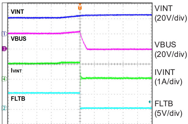
VINT OVP Operation with R_{OVP} = 20\text{k}\Omega
