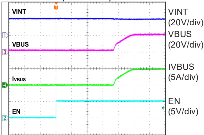
Turn-On by EN (VINT = 20V)
