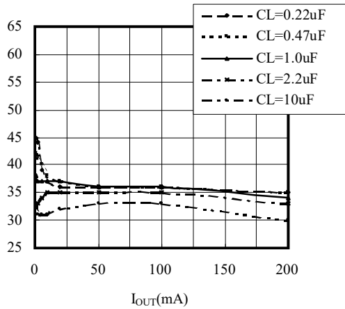
■ Output Noise vs. Output Current C_L =Tantal, C_{NP}=0.01\mu\text{F}
