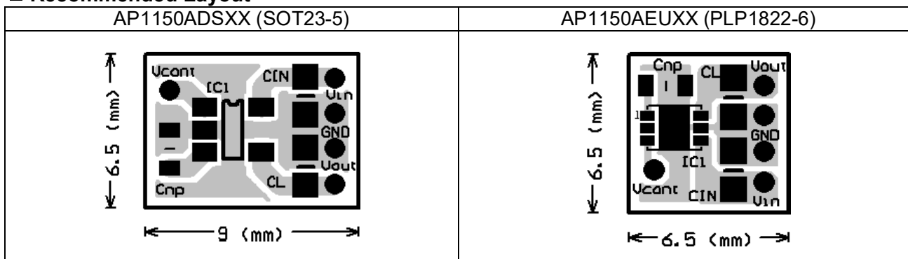
Figure 7. Layout pattern example
