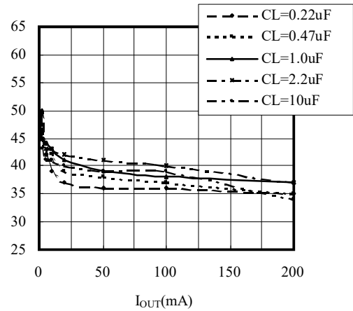
■ Output Noise vs. Output Current C_L =MLCC, C_{NP}=0.01\mu\text{F}
