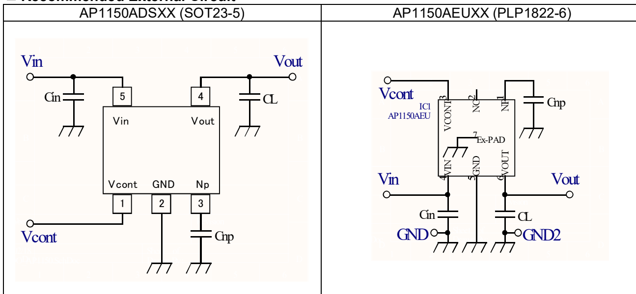
Figure 6. External connection circuit example
