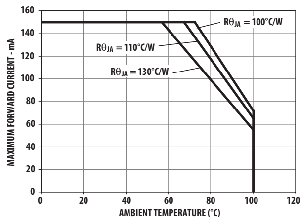
Figure 6a. Maximum Forward Current Vs. Ambient Temperature. Derated Based on T_{JMAX} = 125^\circ\text{C} , R\theta_{JA} = 130^\circ\text{C/W} , 110^\circ\text{C/W} and 100^\circ\text{C/W}
