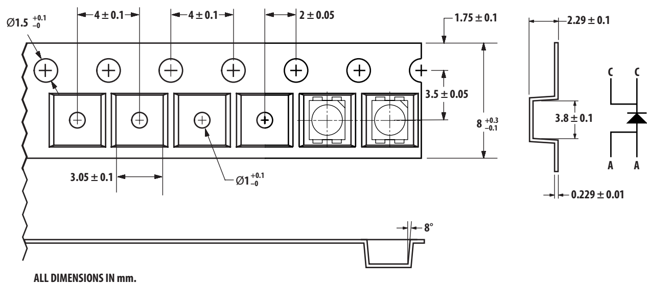
Figure 14. Tape Dimensions
