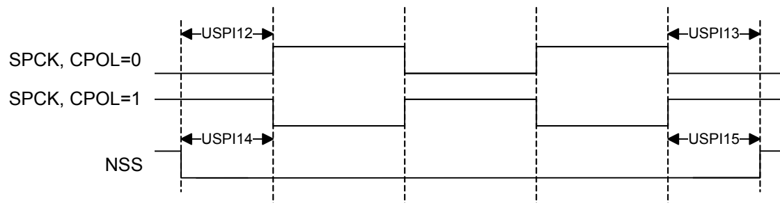
Figure 7-10. USART in SPI Slave Mode NPCS Timing
