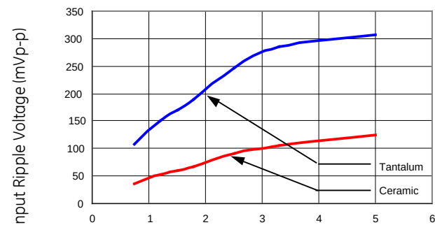
Figure 27. Input ripple voltage for various output with 2x47 µF tantalum capacitors and with 2x22 µF ceramic capacitors at the input (80% of I_{O,max} ).
