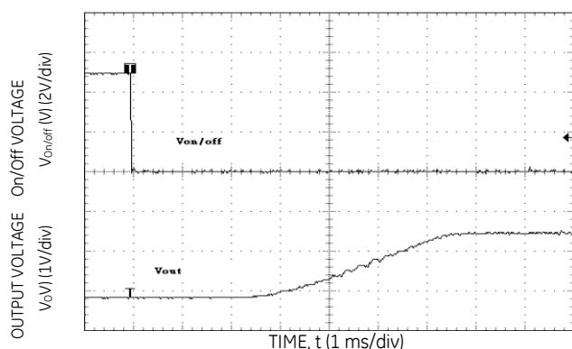
Figure 15. Typical Start-Up Using Remote On/Off with Low-ESR external capacitors (7x150µF Polymer) ( V_{in} = 12 Vdc, V_o = 3.3 Vdc, I_o = 6.0 A, C_o = 1050 µF).
