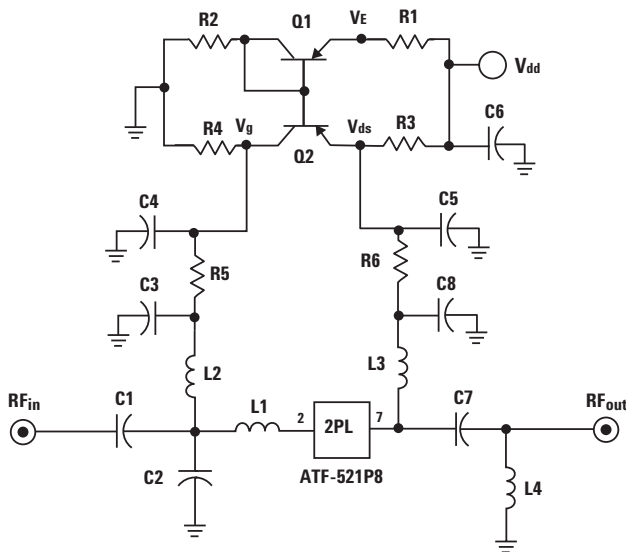
Figure 9. Active Bias Circuit.
