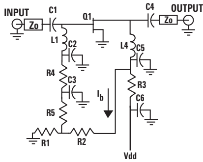
Figure 8. Passive Biasing.
