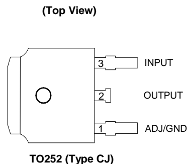
TO252-2
