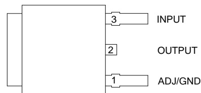
TO252-2
