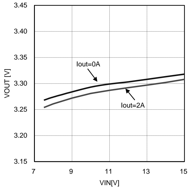
Figure 9. VOUT Line Regulation (VOUT=3.3V, L=3.3μH, Iout=0A / 2A)
