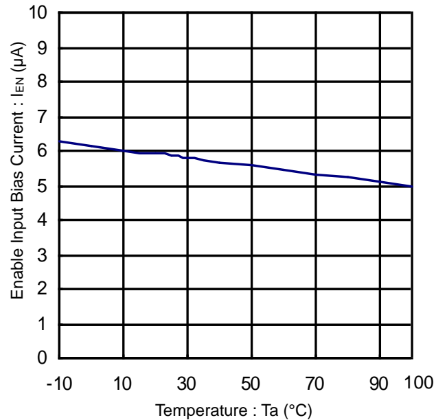
Figure 22. Enable Pin Bias Current vs Temperature
