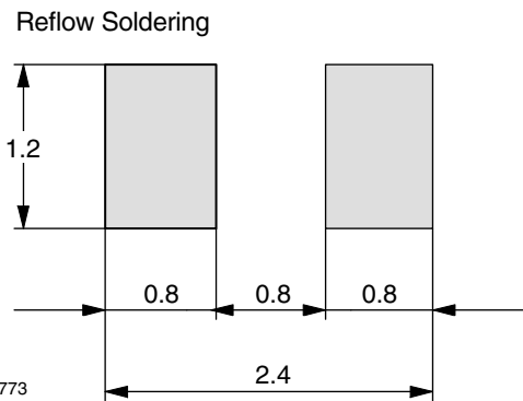
Fig. 11 - Recommended Foot Pads (in mm)
