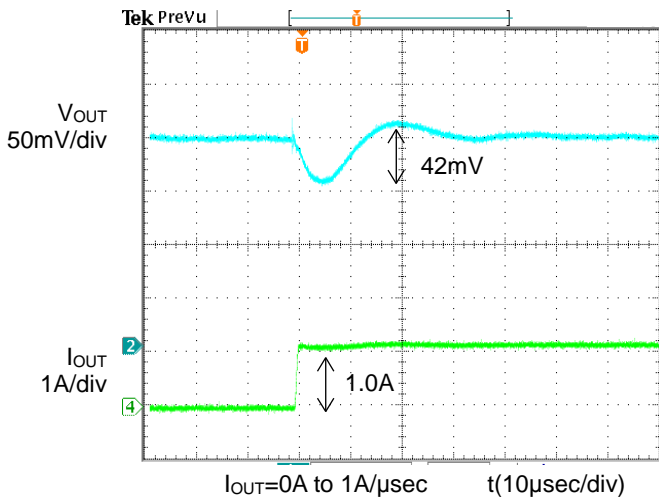
Figure 7. Transient Response (0A to 1.0A) C_{OUT}=100\mu F, C_{FB}=1000pF
