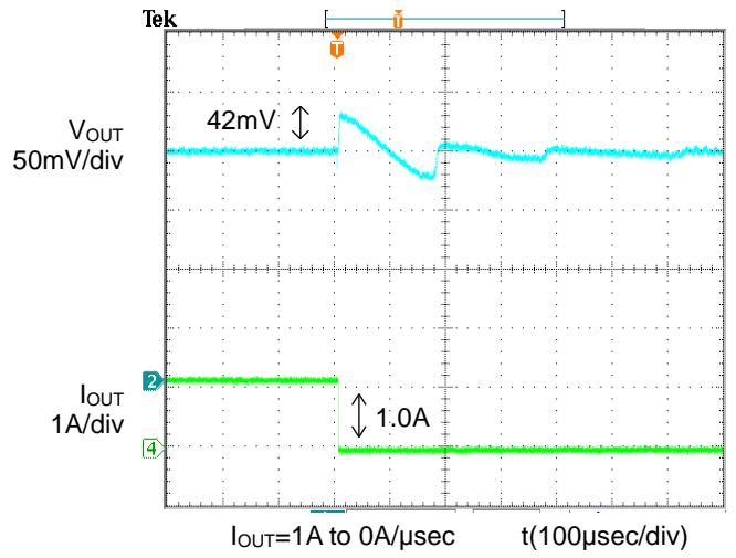
Figure 10. Transient Response (1.0A to 0A) C OUT =100µF, C FB =1000pF
