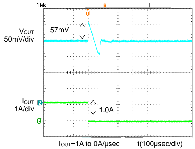
Figure 12. Transient Response (1.0A to 0A) C OUT =22µF, C FB =1000pF
