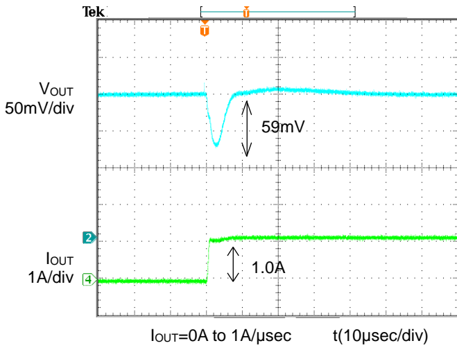
Figure 9. Transient Response (0A to 1.0A) C OUT =22µF, C FB =1000pF
