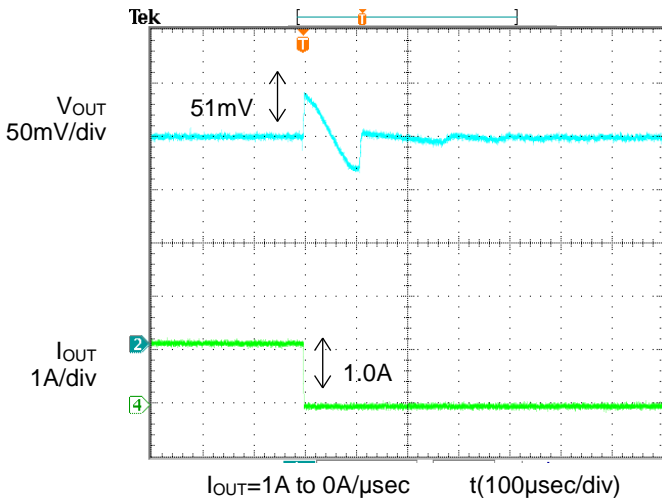
Figure 11. Transient Response (1.0A to 0A) C OUT =47µF, C FB =1000pF
