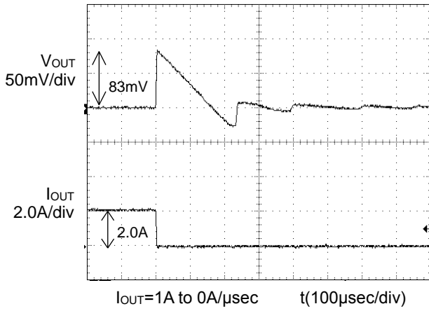
Figure 17. Transient Response (2.0A to 0A) C_{OUT}=47\mu F , C_{FB}=1000pF
