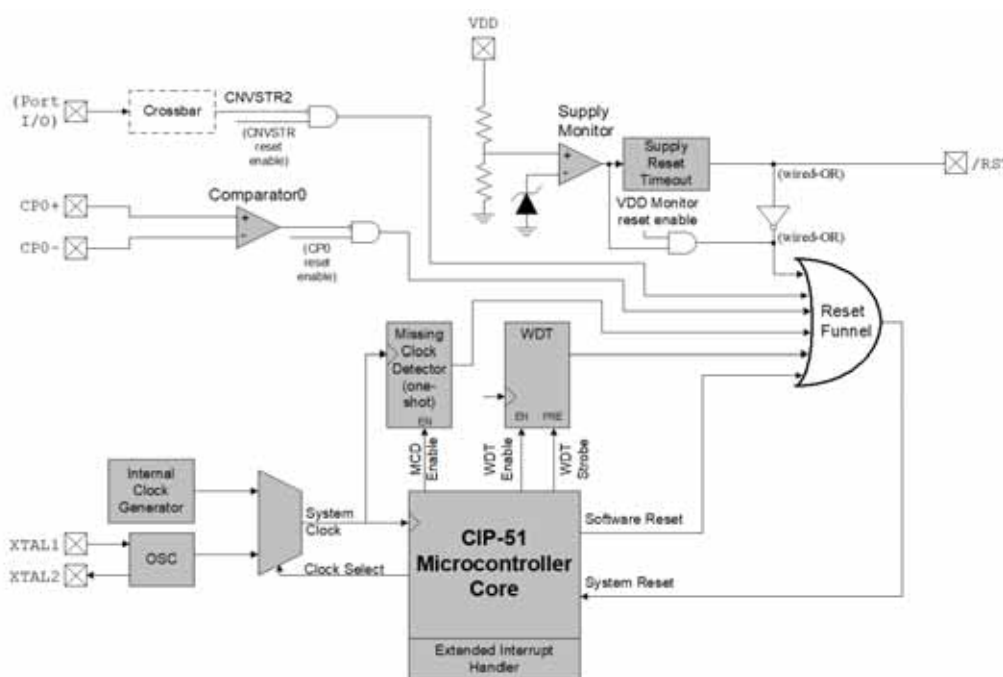
Figure 14.1. Reset Sources
