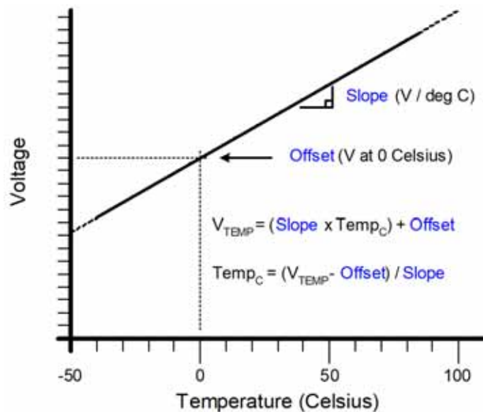
Figure 7.2. Temperature Sensor Transfer Function
