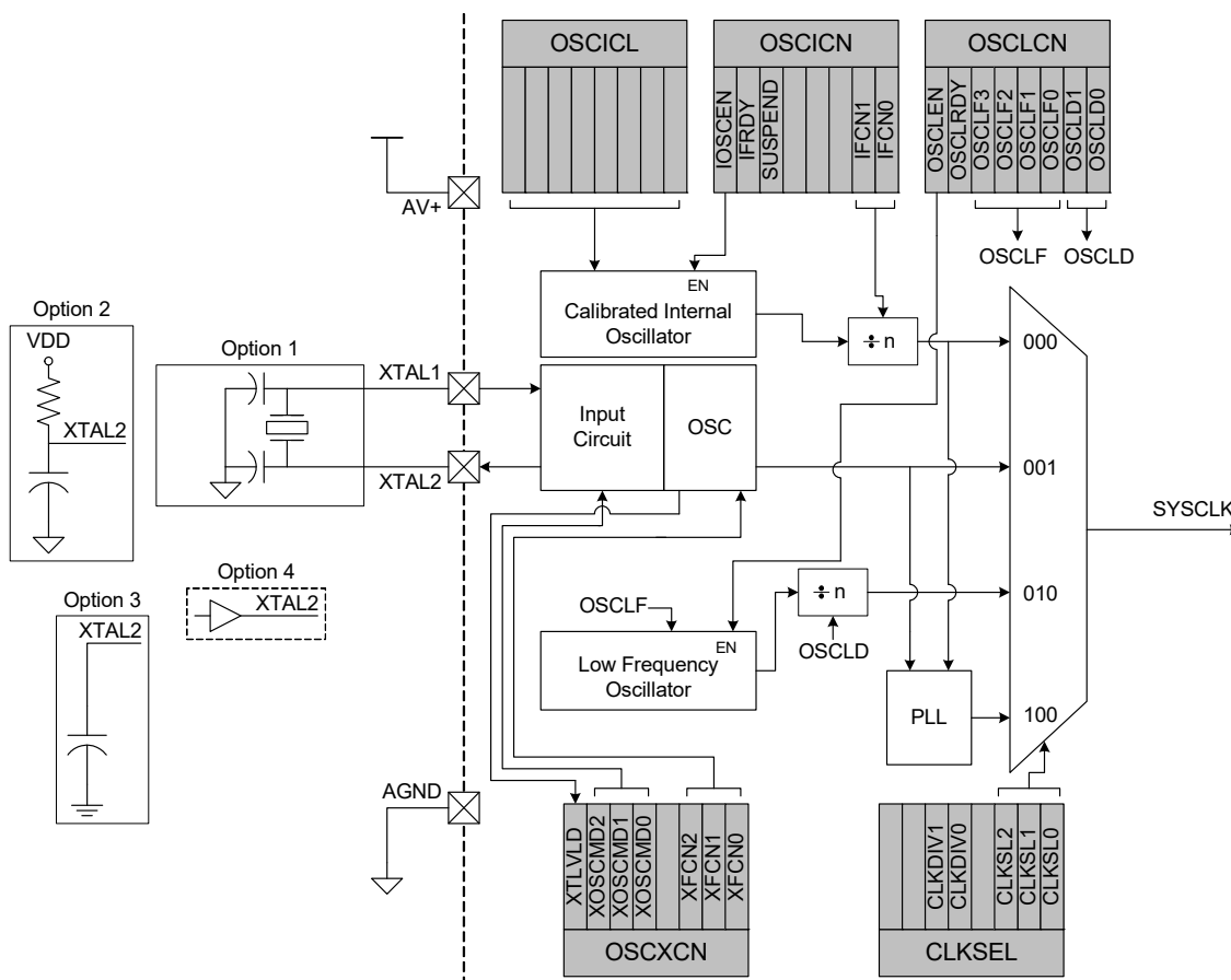
Figure 16.1. Oscillator Diagram
