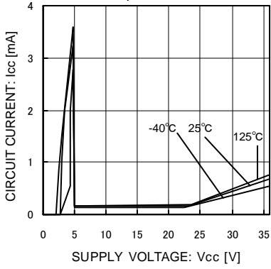
Fig.1 Circuit Current
