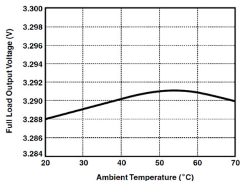
Figure 13. Regulator V_{OUT} vs. T_{AMB} (250 mA Load)
