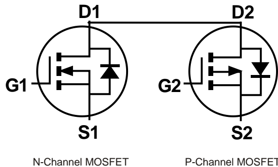
Equivalent Circuit
