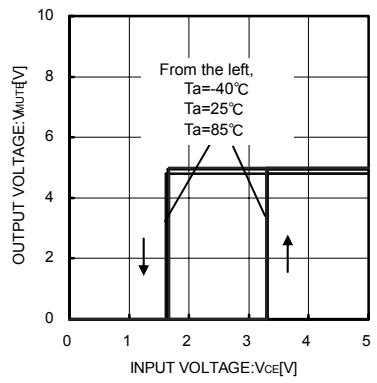
Fig.40 CE-CMP Threshold 2 (SEL = H)
