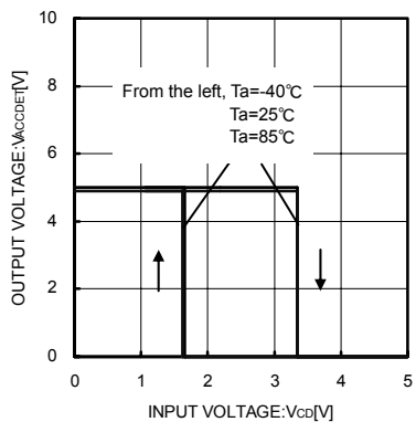
Fig.43 CD-CMP Threshold 2 (SEL = H)
