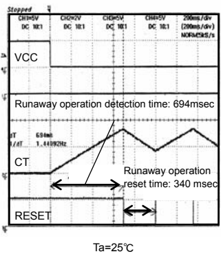
Fig.47 Runaway Operation RESET Time
