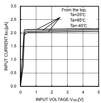
Fig.18 SEL Input Current
