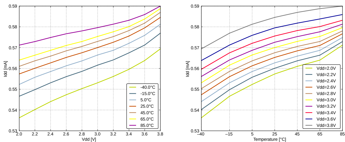
Figure 4.9. EM1 Current Consumption with all Peripheral Clocks Disabled and HFRCO Running at 11 MHz
