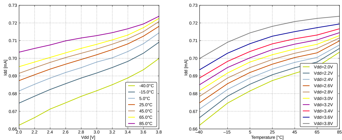
Figure 4.8. EM1 Current Consumption with all Peripheral Clocks Disabled and HFRCO Running at 14 MHz
