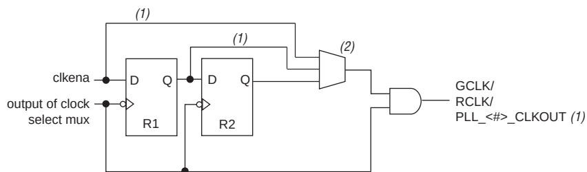
Figure 6-16. clkena Implementation
