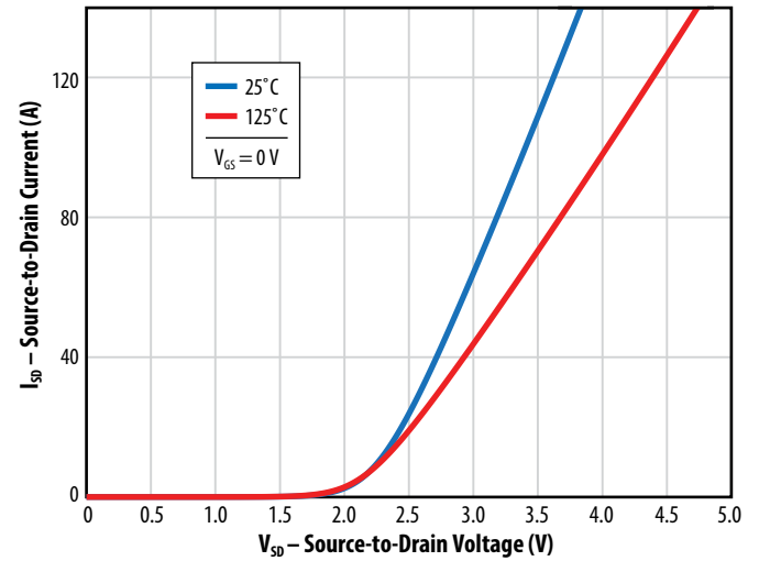
Figure 8b (Q2): Reverse Drain-Source Characteristics
