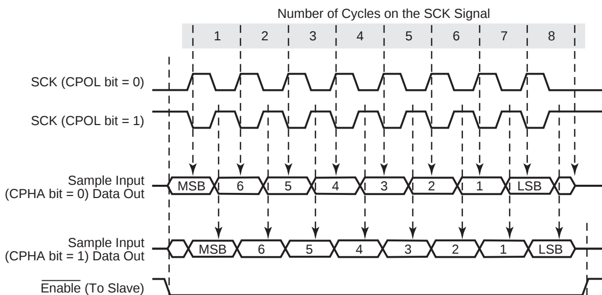
Figure 29. SPI Timing
