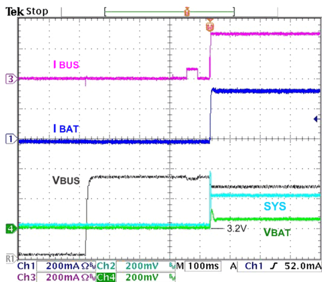
Figure 13. Charger Startup at V_{\text{BUS}} Plug-In Using 300 mA Current Limited Source, 500 mA I_{\text{BUSLIM}} , 3.2 V V_{\text{BAT}} , 50 \Omega SYS Load
