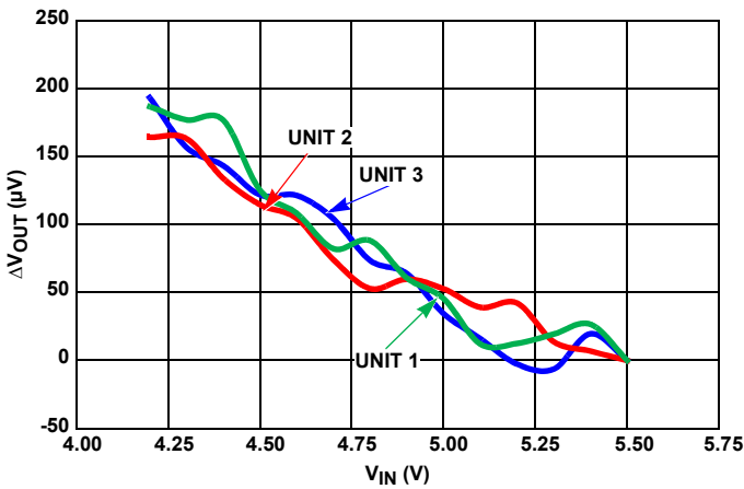
FIGURE 124. LINE REGULATION, THREE UNITS
