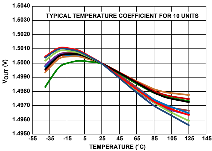
FIGURE 51. V_{OUT} vs TEMPERATURE
