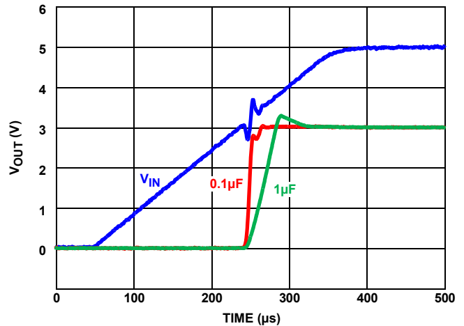
FIGURE 97. TURN-ON TIME
