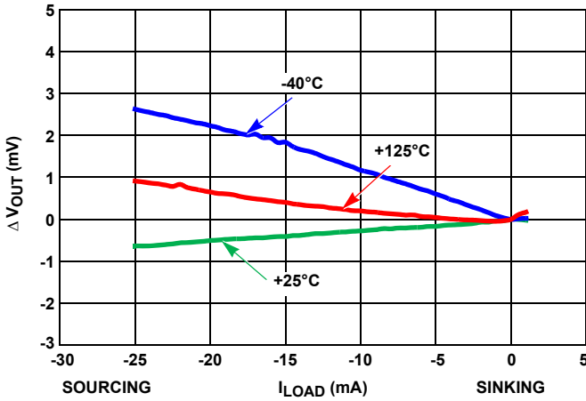
FIGURE 60. LOAD REGULATION OVER-TEMPERATURE
