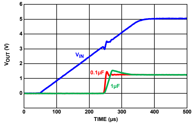
FIGURE 29. TURN-ON TIME
